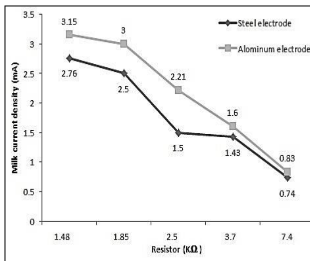
Fig 3 Chart of changes in the electrical current density of the aluminum and steel electrodes in terms of the circuit resistor, with the equal cell coefficient in two minutes at 17.2 ° C and 15 cc of milk.
