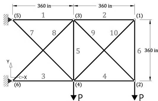
Figure 2. 10-bar truss
