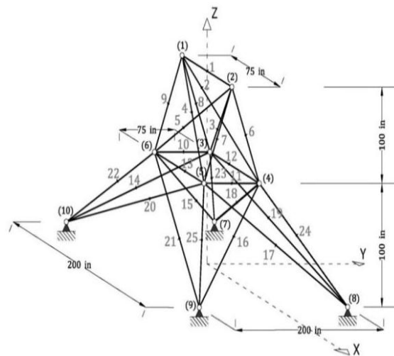
Figure 4. 25-bar spatial truss
