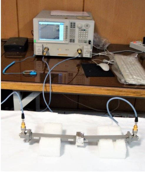
Fig. 3: Measurement system, vector network analyzer.
