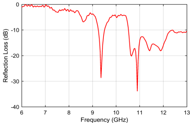
Fig. 6: Reflection loss of \text{RAM-TiO}_2@MWCNT/\text{Fe}_3\text{O}_4/\text{PANI} .
