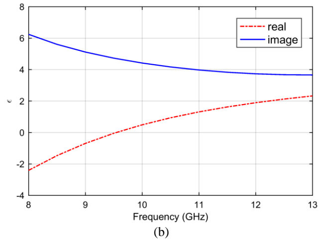
Fig. 4: (a) Complex permeability and (b) Complex permittivity of \text{TiO}_2\text{@MWCNT/Fe}_3\text{O}_4\text{/PANI} -epoxy absorbers.
