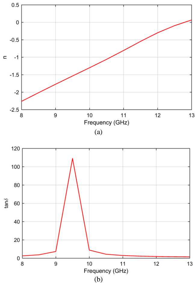
Fig. 5: (a) Refraction coefficient and (b) dielectric loss tangent for the \text{TiO}_2@MWCNT/\text{Fe}_3\text{O}_4/\text{PANI} -epoxy absorbers
